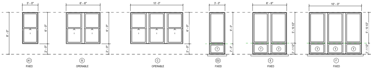
Vinyl Window, double pane Low-E
